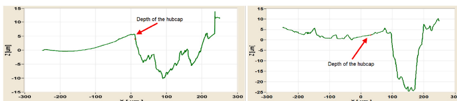
Fig. 6. 2D profile of the worn region of the fly ash samples region with more accentuated wear and formation of valleys.
