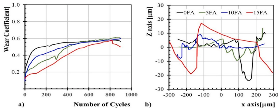
Fig. 5. a) Composite wear test with different cycles. b) In effect on the X and Z axes.
