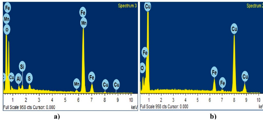
Fig. 4. EDS of the composites of sintered samples. a) Composite A with fly ash. b) Composites without fly ash.
