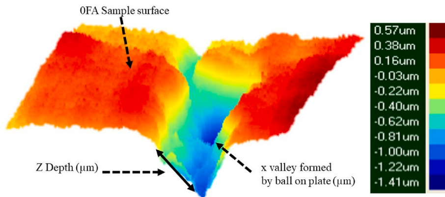
Fig. 7. Profilometric test results in 3D. In the red region with homogeneous wear. Blue region with more accentuated wear and valley formation. (For interpretation of the references to color in this figure legend, the reader is referred to the Web version of this article.)
