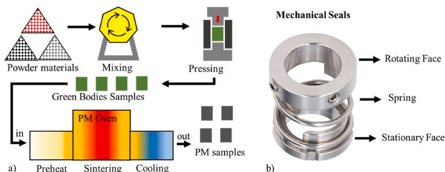
Fig. 1. PM process in a) and the manufacture of mechanical seals in b).
