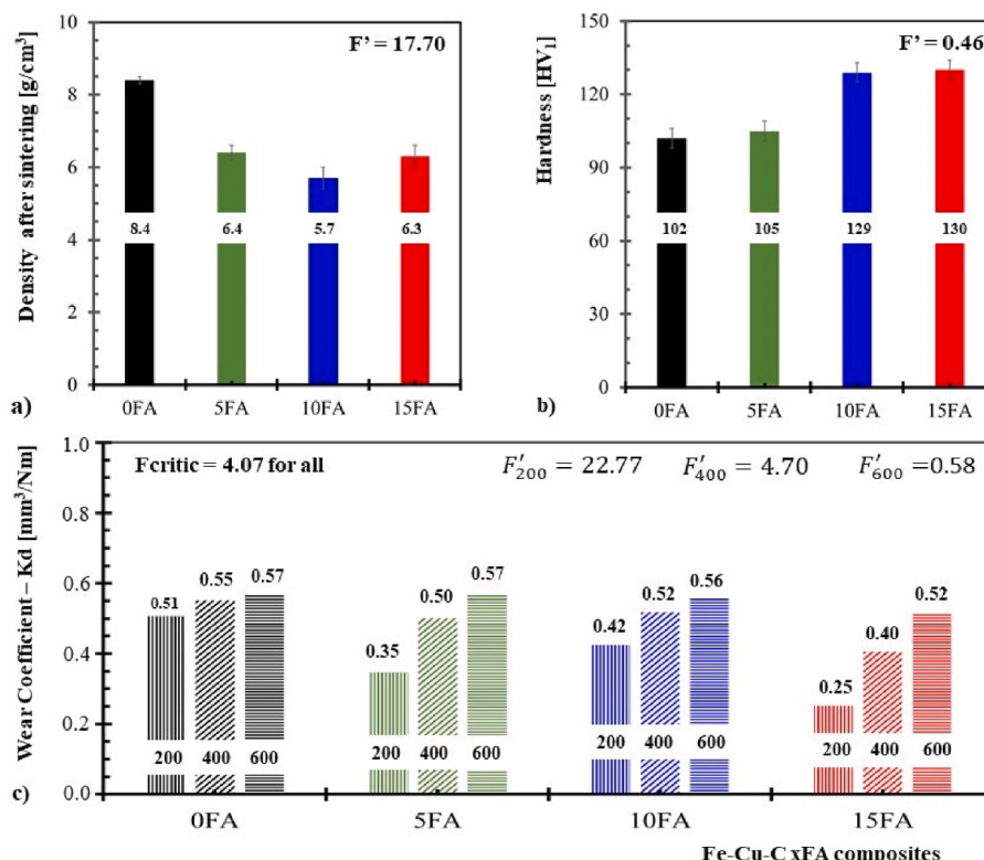
Fig. 8. Analysis of variance of the results obtained, density a), microhardness b), and wear coefficient in c).
