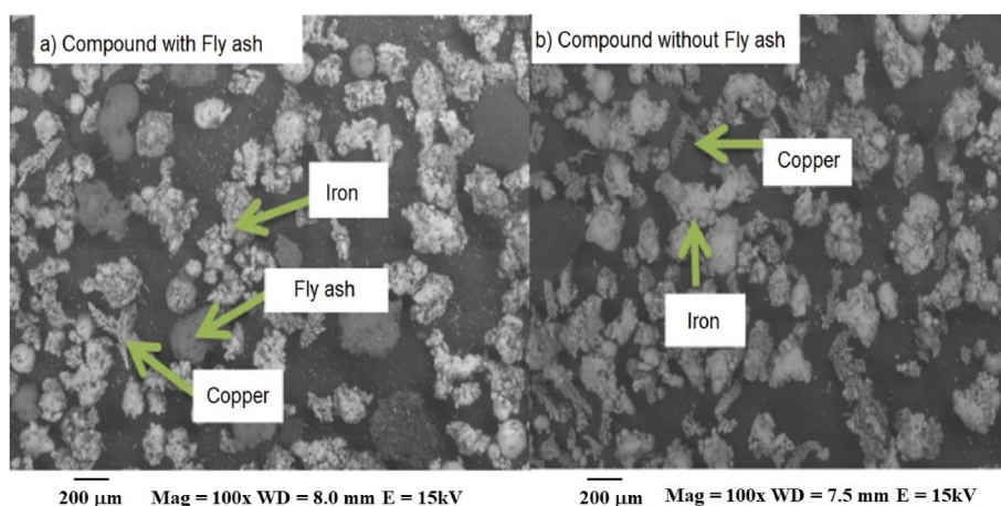
Fig. 3. Matrix and chemical distribution of composites - sintered sample: a) Compound A with ash. b) Compound without ash.
