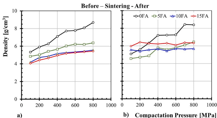
Fig. 2. Density before a) and after sintering b).
