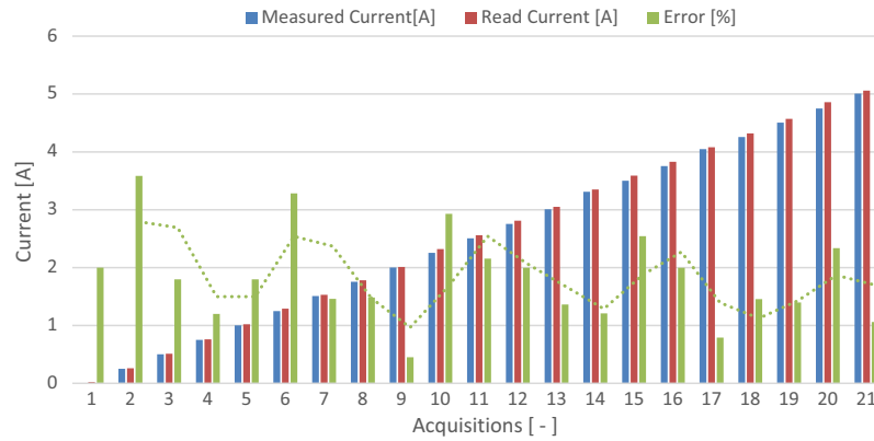
Fig. 6. Current curve without adjustment.
