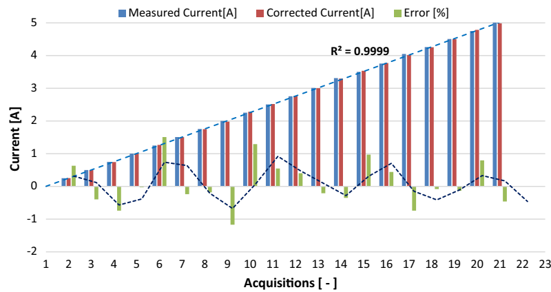
Fig. 7. Current curve with adjustment.
