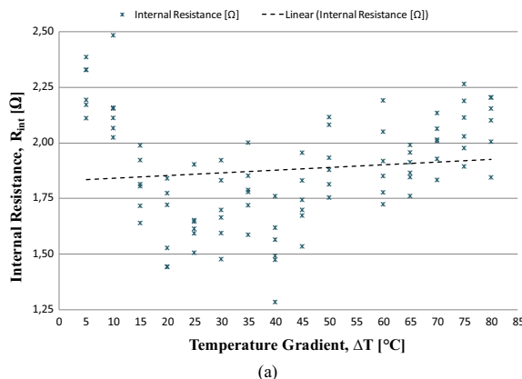
Fig. 13. (a) The internal resistance of TEG, R_{int} [ \Omega ], as function of the temperature gradient, \Delta T [°C]. (b) The medium and standard deviation values of the internal resistance of TEG, R_{int} [ \Omega ], as function of the temperature gradient, \Delta T [°C].
