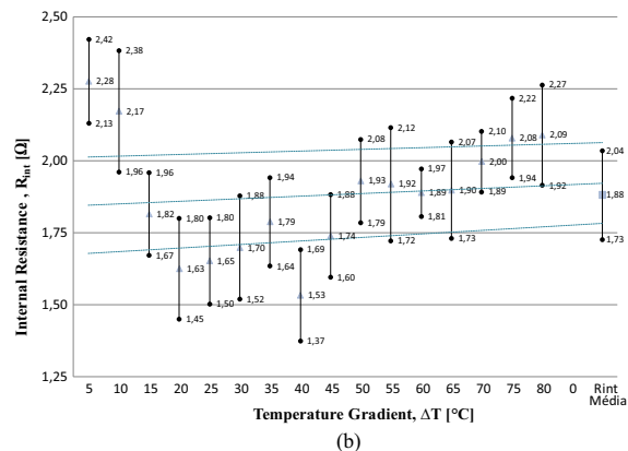
Fig. 13. (a) The internal resistance of TEG, R_{int} [ \Omega ], as function of the temperature gradient, \Delta T [°C]. (b) The medium and standard deviation values of the internal resistance of TEG, R_{int} [ \Omega ], as function of the temperature gradient, \Delta T [°C].
