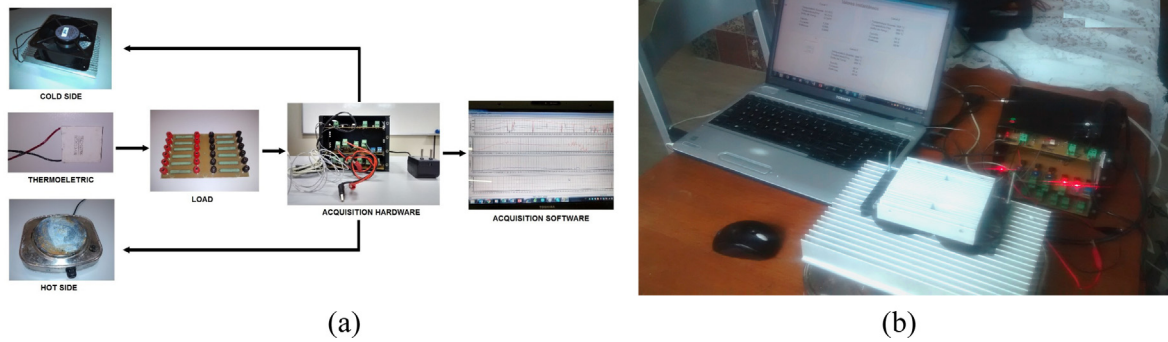
Fig. 11. Diagram system mounting blocks (a) and assembled experiment (b).
