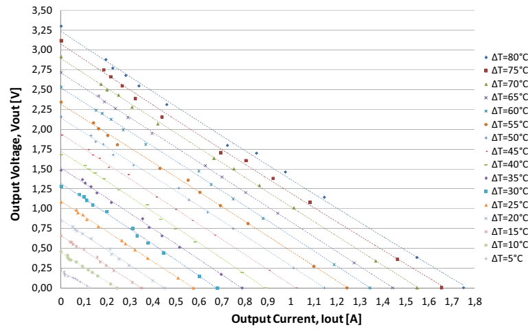
Fig. 14. The output voltage, V_{out} [V] versus the output current, I_{out} [A], for different temperature gradient, \Delta T [°C].
